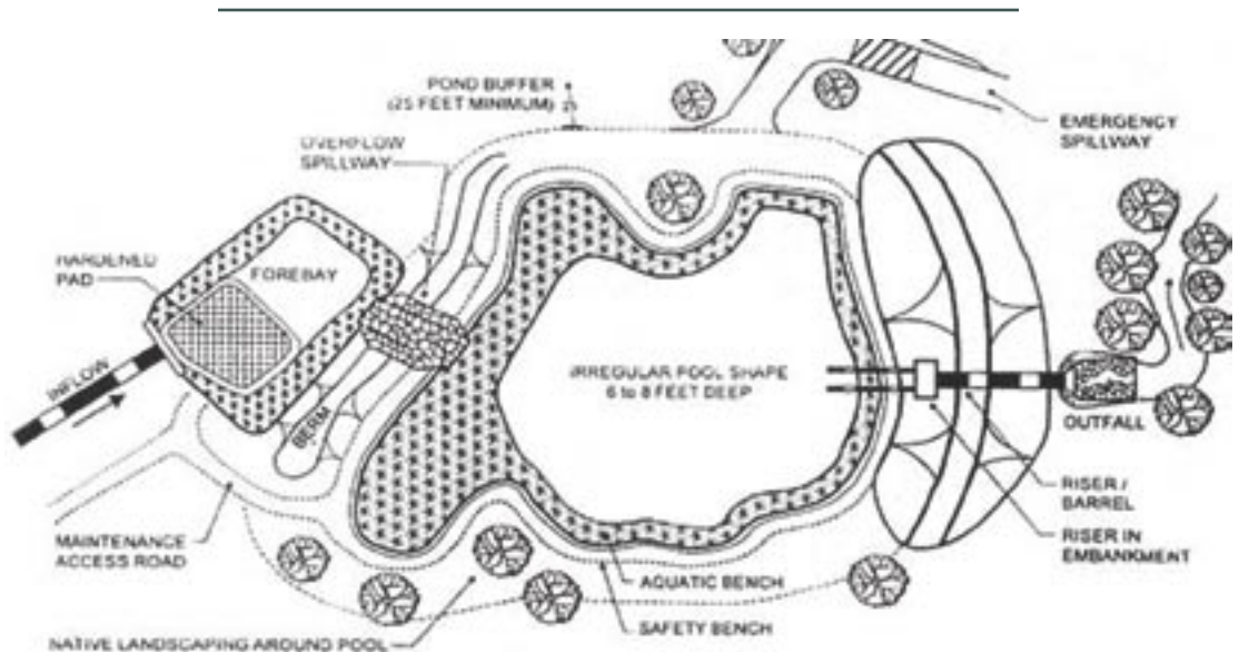
Figure 6-4. Example of a wet detention pond. Source: Center for Watershed Protection 1998.
