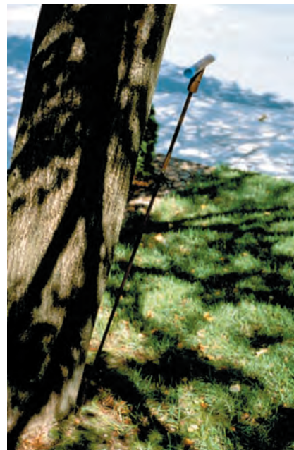
Figure 3.155. A metal probe inserted into the soil near the root collar.
